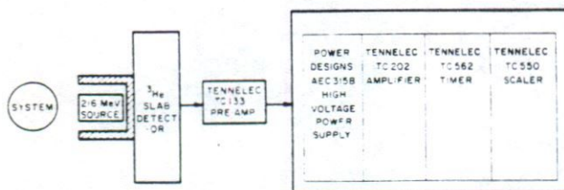
Fig. 10. Block diagram, ( \gamma, n ) system.
